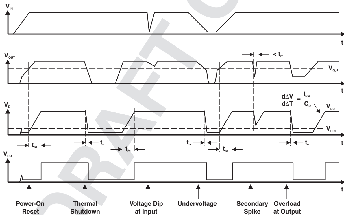
Figure 2. Reset Timing
