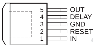
KTT PACKAGE (TOP VIEW)
